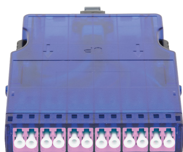
NMF-CJ12M4PA-MTPM-LCU-1S 1 slot, MM 50/125 OM4, 1x MTP / male - 12x LC / UPC, полярность A
